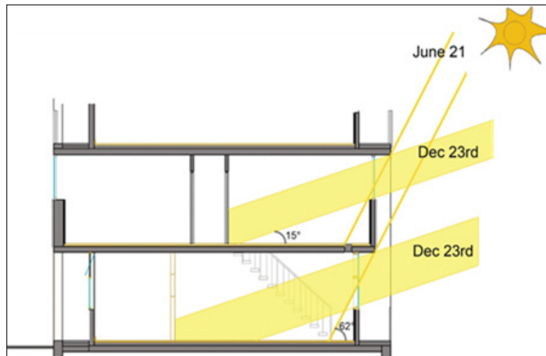
Figure 37: Illustration of sun ingress during Summer and Winter solstice.
