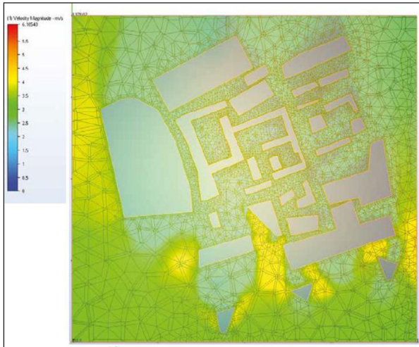
Figure 22: CFD simulation showing wind pattern.
